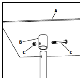
-Detail 1- Assembling inspection panel to post.
