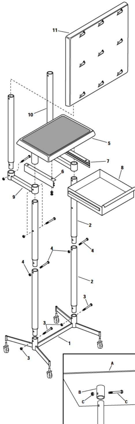
-Detail 1- Assembling inspection panel to posts.
